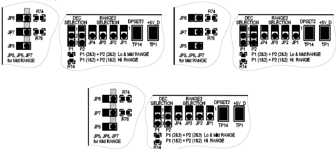
Figure 3-7. Configuration Jumper Settings
